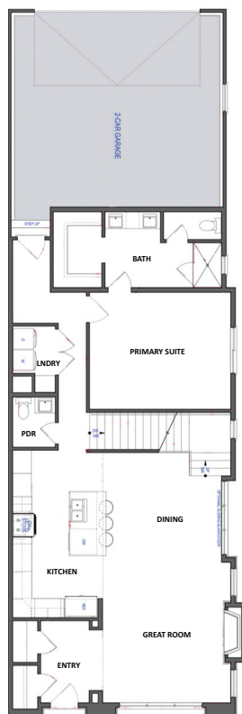
main floor 1,328 sq ft
