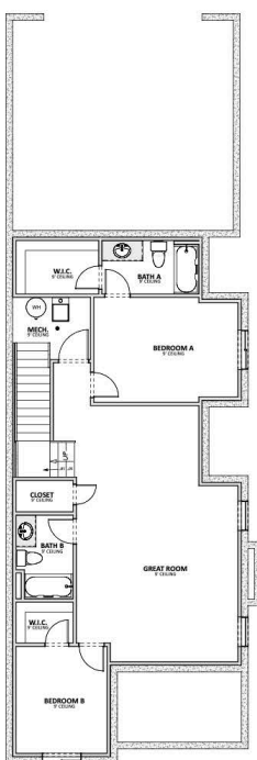
opt. finished basement 1,162 sq ft
