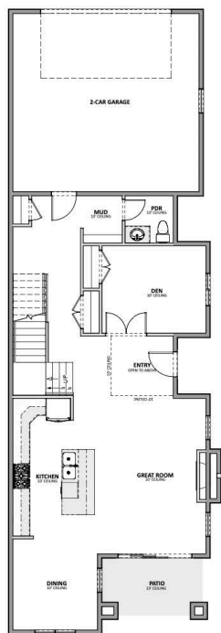
main floor 1,162 sq ft
